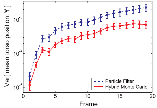
Figure 9. Estimator variance for estimates of the mean torso position over a 20-frame sequence. The vertical bars indicate one standard error, obtained from 40 independent runs of the filter.
